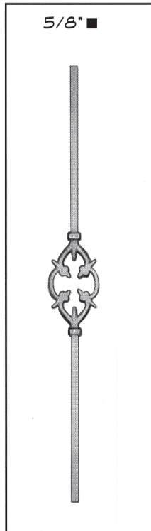
158 HEIGHT: 37 1/4" 94.62 cm WIDTH: 4 1/2" 11.43 cm THICK: 1 1/8" 2.54 cm WEIGHT: 2.4 lbs 6.10 kgs
