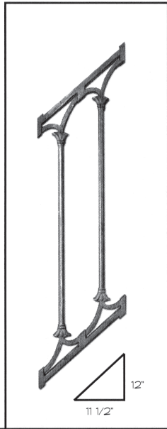
937 HEIGHT: 37" 93.98 cm WIDTH: 8" 2.54 cm THICK: 5/8" 0.625 cm WEIGHT: 3.3 lbs 8.38 kgs
